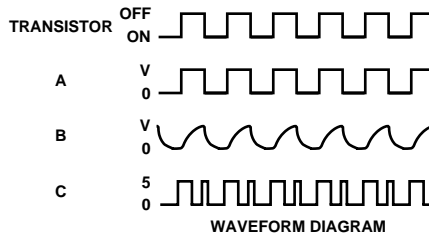
Figure 12. Frequency Doubler
