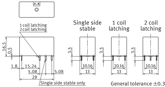
External dimensions
