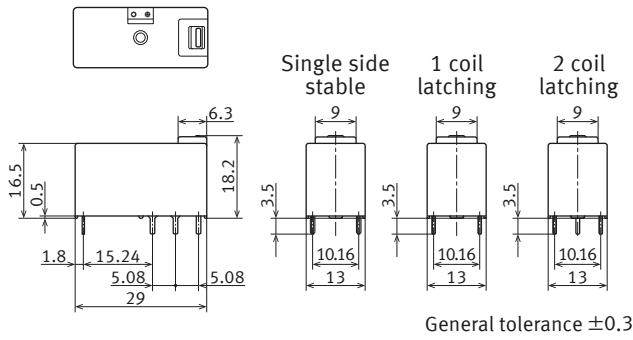
External dimensions
