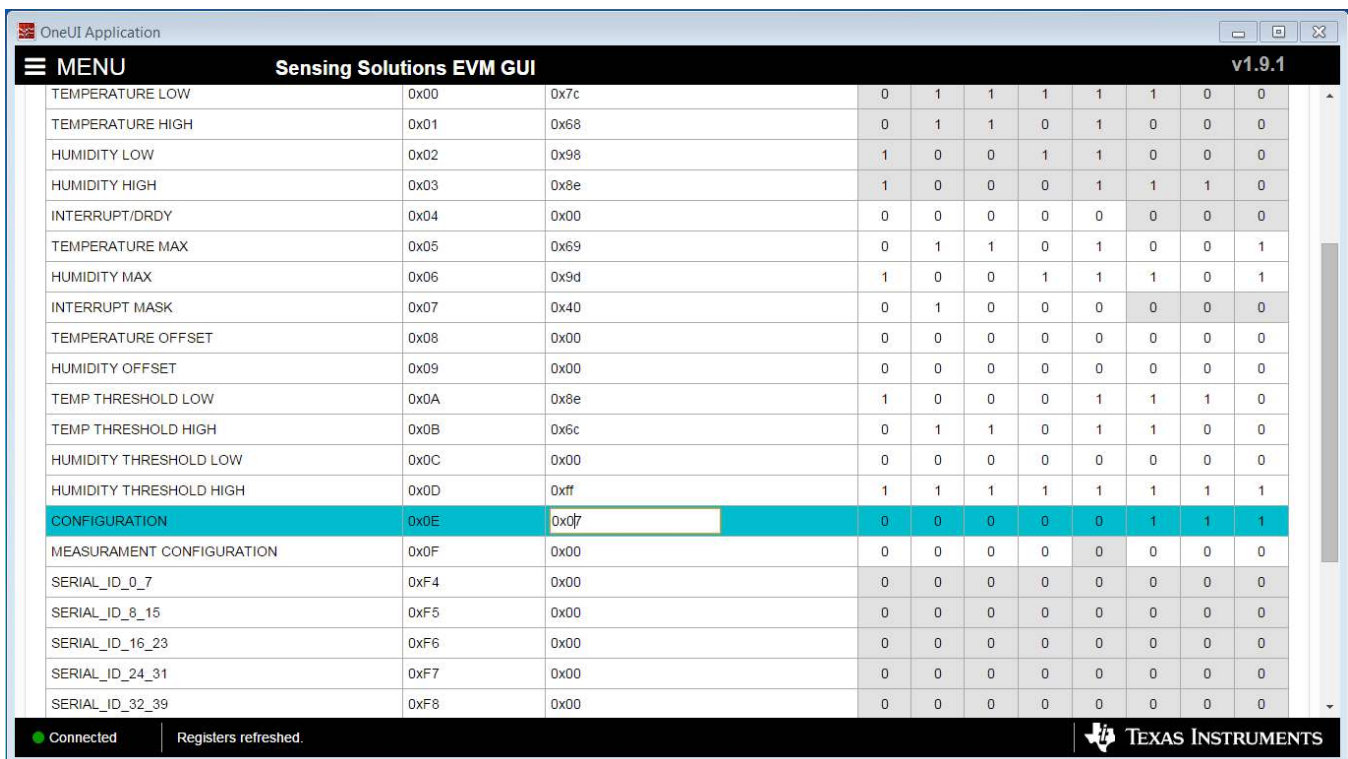
Figure 23. Entering New Value for Register on Register Page
