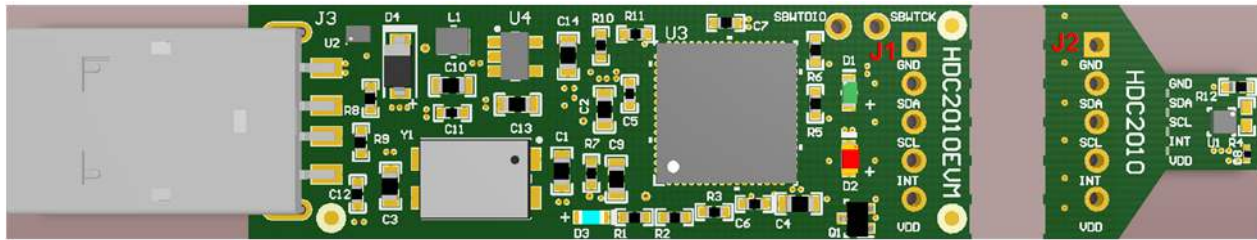
Figure 12. HDC2010EVM : PC Interface and Sensor Module
