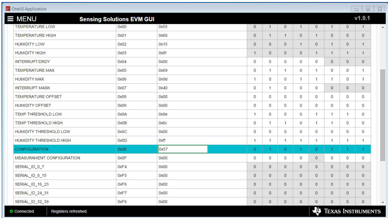
Figure 22. Selecting a Register's Current Value for Editing on Register Page
