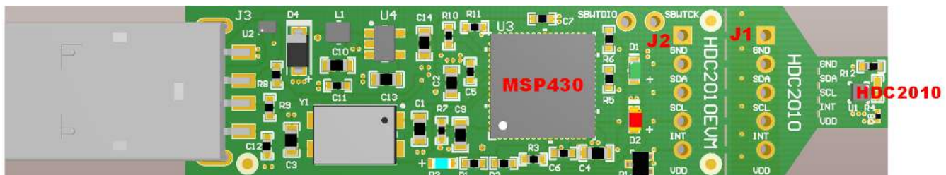
Figure 1. HDC2010EVM
