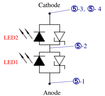
Inside circuit
