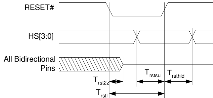
Figure 1. \overline{\text{RESET}} Timing
