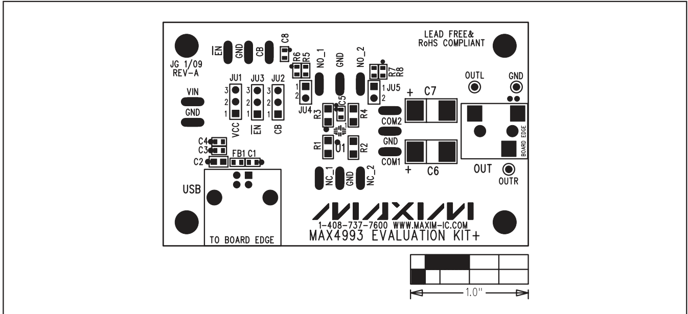
Figure 2. MAX4993 EV Kit Component Placement Guide—Component Side
