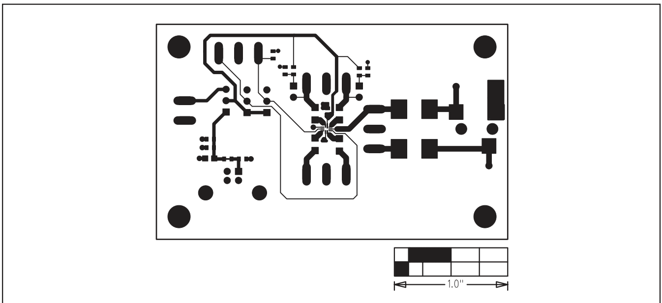
Figure 3. MAX4993 EV Kit PCB Layout—Component Side
