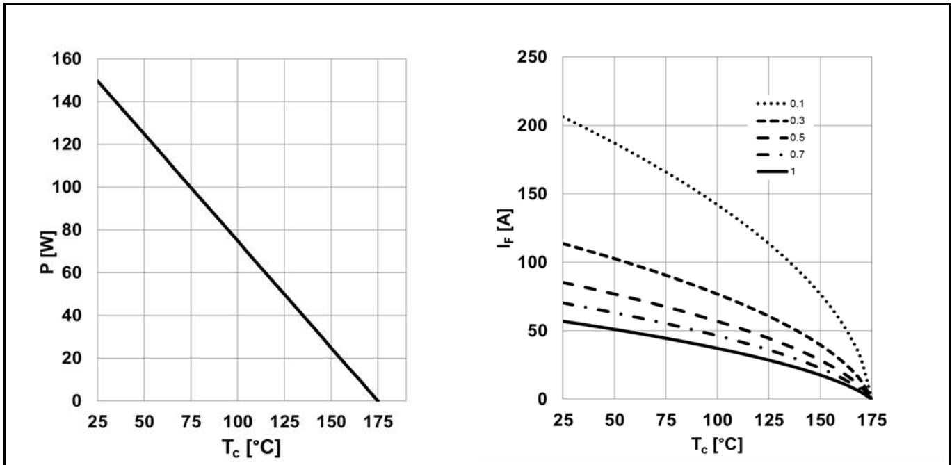
Figure 1 (LEFT) Power dissipation; P_{tot} = f(T_c) ; R_{thJC,max} (RIGHT) Diode forward current; I_F = f(T_c) ; T_j \leq 175^\circ C ; R_{thJC,max} ; parameter: D=duty cycle
