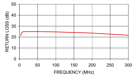
TC3-1TG2+ INPUT RETURN LOSS
