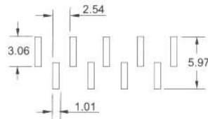
PC Board Layout
