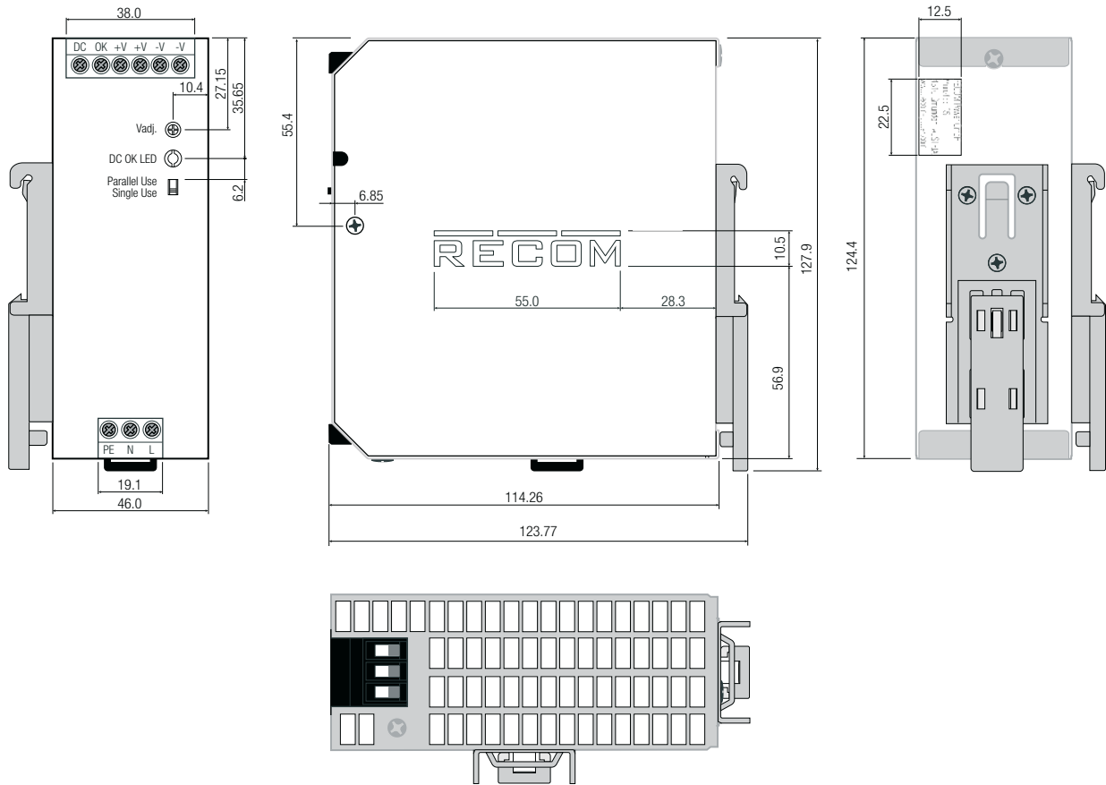
Dimension Drawing (mm)
