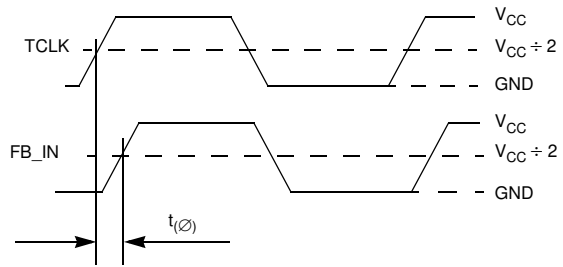
Figure 15. Propagation Delay ( t_0 ) Test Reference
