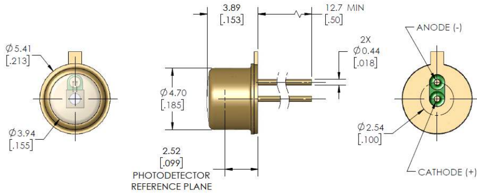
Figure 2: TO-18 Dimensions C30902EH
