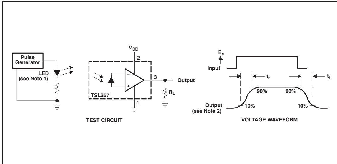
Figure 10: Switching Times
