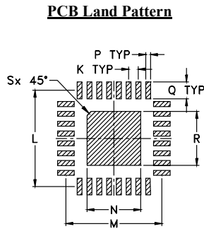
Suggested Layout, Tolerance to be within ±.002
