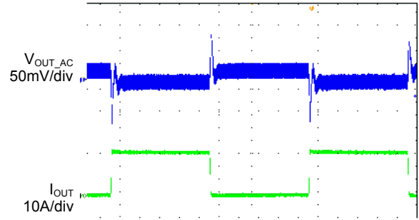
Time 400µs/div
