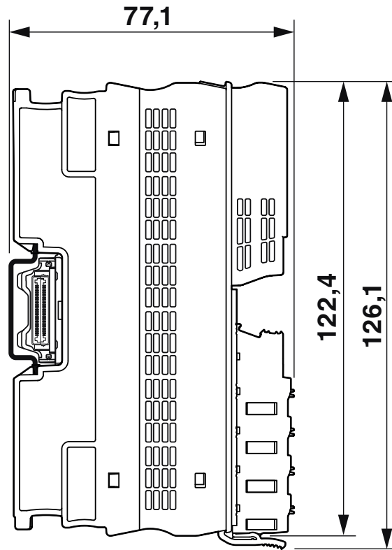
Dimensional drawing
