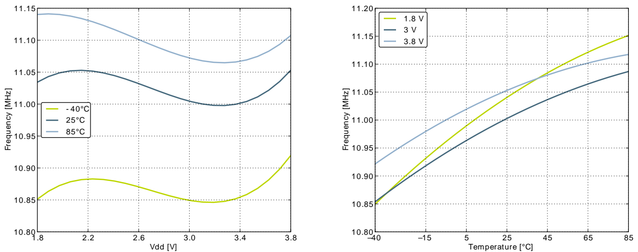
Figure 3.24. Calibrated HFRCO 14 MHz Band Frequency vs Supply Voltage and Temperature
