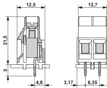
Dimensioned drawing
