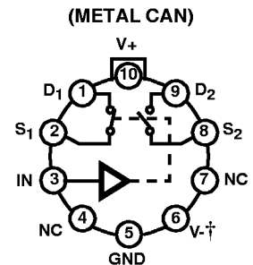
SPST HI-301 AND HI-305 TOP VIEWS
