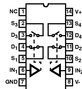
DUAL SPDT HI-303 AND HI-307 (PDIP, CERDIP, SOIC) TOP VIEW
