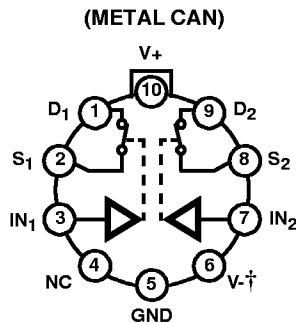
DUAL SPST HI-300 AND HI-304 TOP VIEWS
