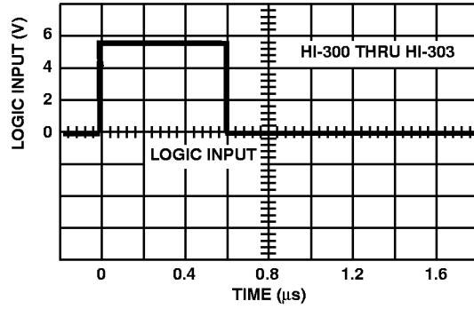
FIGURE 7B. V_{IN(Logic)} vs TIME
