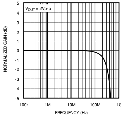
MAX4105 LARGE-SIGNAL GAIN vs. FREQUENCY ( A_{VCL} = +5 )
