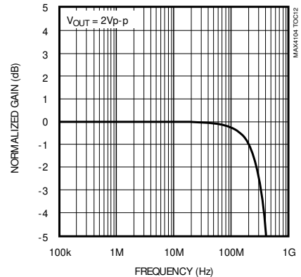
MAX4305 LARGE-SIGNAL GAIN vs. FREQUENCY ( A_{VCL} = +10 )
