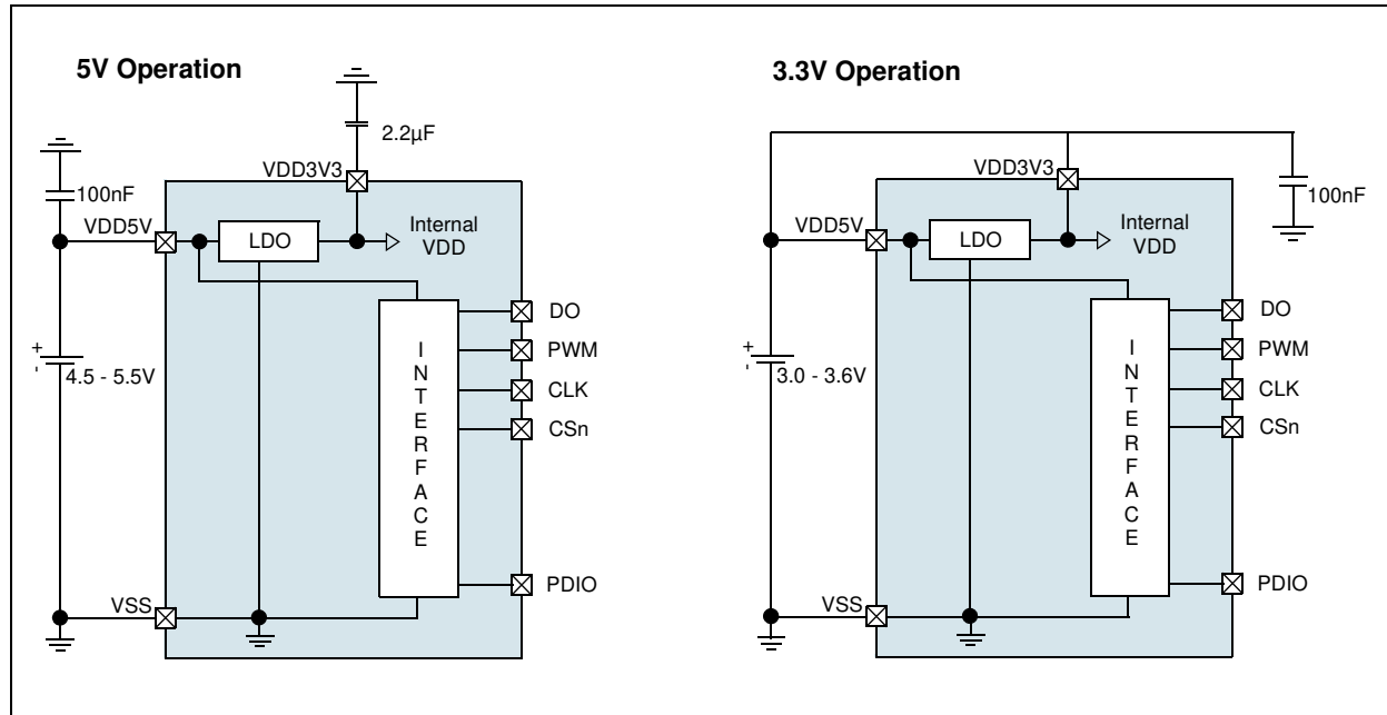
Figure 16. Connections for 5V / 3.3V supply voltages
