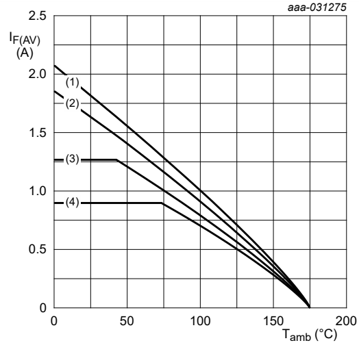
FR4 PCB, standard footprint T_j = 175\text{ }^\circ\text{C} (1) \delta = 1 ; DC (2) \delta = 0.5 ; f = 20 kHz (3) \delta = 0.2 ; f = 20 kHz (4) \delta = 0.1 ; f = 20 kHz
