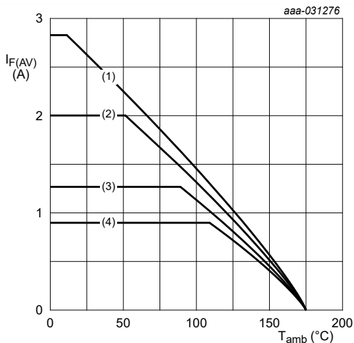
FR4 PCB, mounting pad for cathode 1\text{ cm}^2 T_j = 175\text{ }^\circ\text{C} (1) \delta = 1 ; DC (2) \delta = 0.5 ; f = 20 kHz (3) \delta = 0.2 ; f = 20 kHz (4) \delta = 0.1 ; f = 20 kHz
