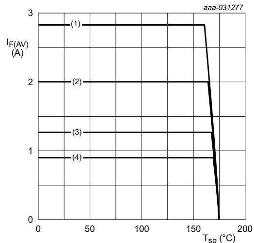
T_j = 175\text{ }^\circ\text{C} (1) \delta = 1 ; DC (2) \delta = 0.5 ; f = 20 kHz (3) \delta = 0.2 ; f = 20 kHz (4) \delta = 0.1 ; f = 20 kHz
