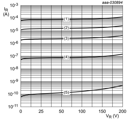
pulsed condition (1) T_j = 175^\circ\text{C} (2) T_j = 150^\circ\text{C} (3) T_j = 125^\circ\text{C} (4) T_j = 85^\circ\text{C} (5) T_j = 25^\circ\text{C}
