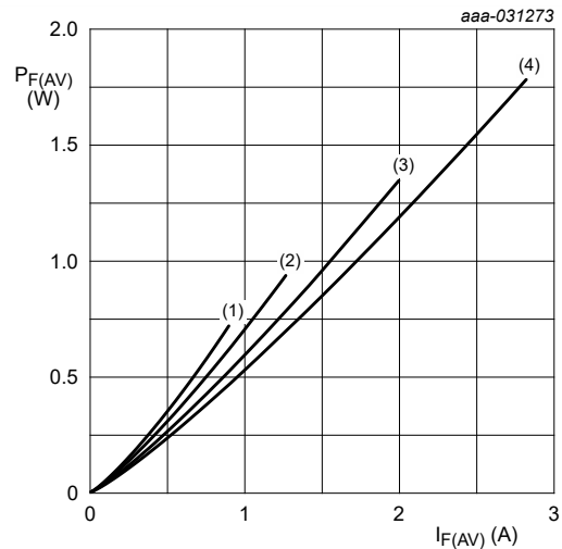
T_j = 175^\circ\text{C} (1) \delta = 0.1 (2) \delta = 0.2 (3) \delta = 0.5 (4) \delta = 1 ; DC
