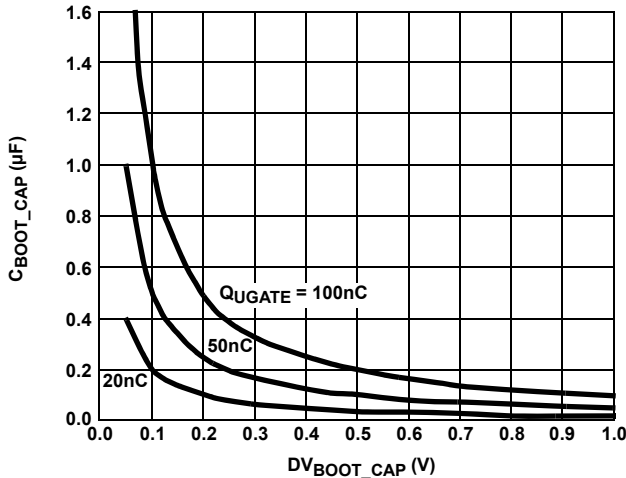
FIGURE 3. BOOTSTRAP CAPACITANCE vs BOOT RIPPLE VOLTAGE
