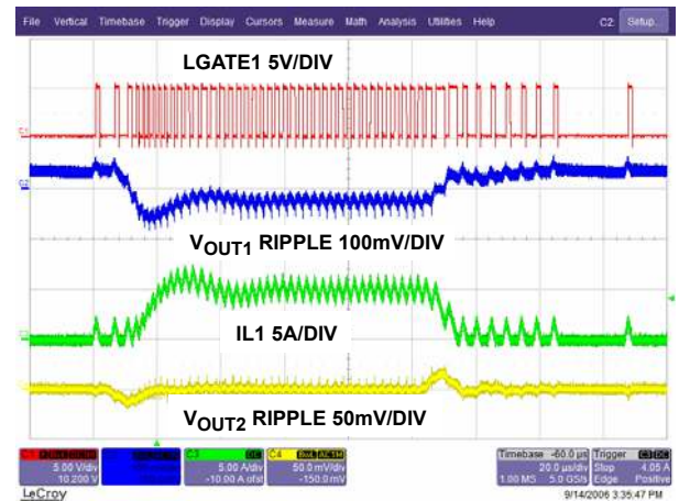
FIGURE 48. LOAD TRANSIENT V_{OUT1} = 5V (SKIP)
