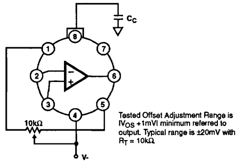
FIGURE 1. SUGGESTED V OS ADJUSTMENT AND COMPENSATION HOOK UP
