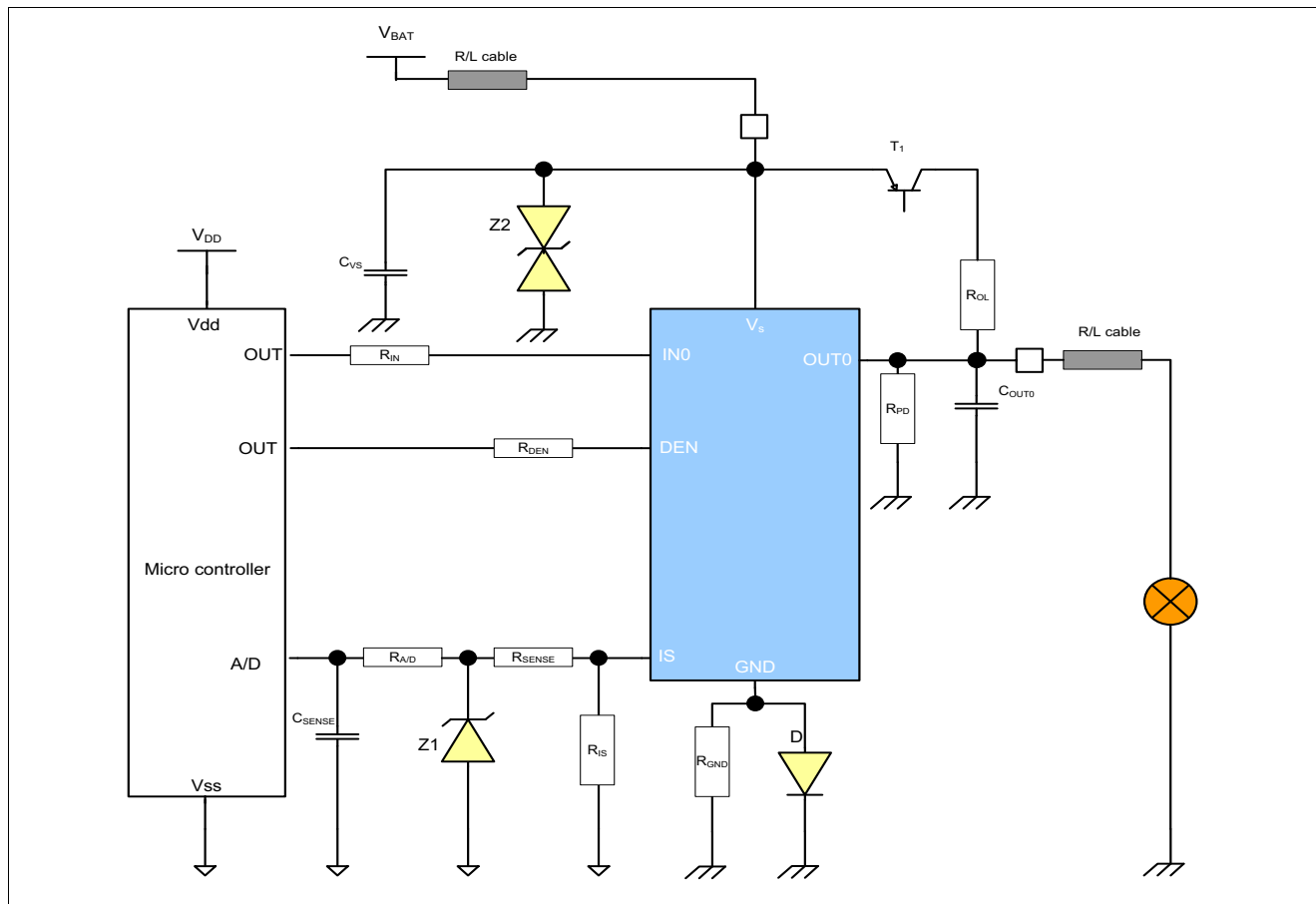
Figure 52 Application Diagram with BTS5010-1EKB
