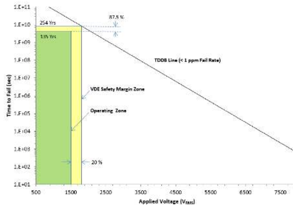
Figure 6-4. Reinforced Isolation Capacitor Lifetime Projection
