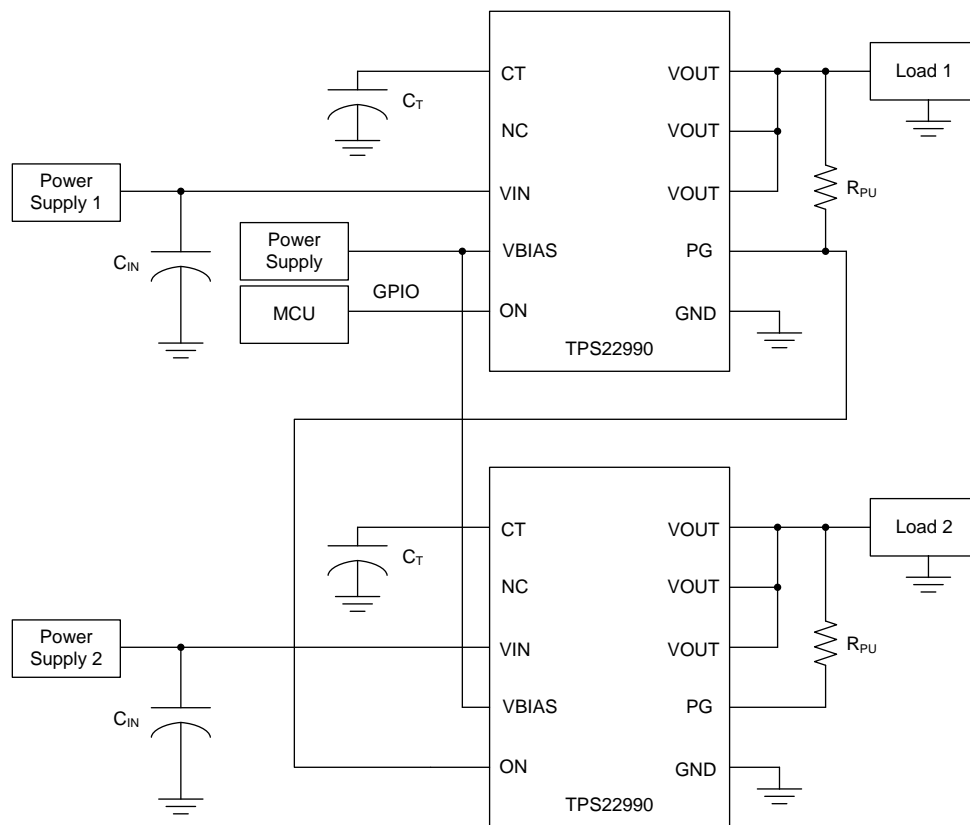
Figure 36. Power Sequencing
