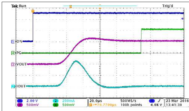
Figure 39. . Inrush Current with C_T = 0 pF
