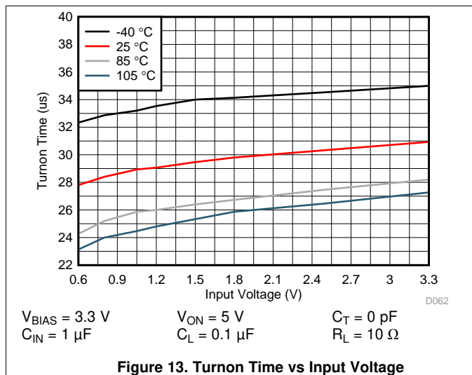
Figure 13. Turnon Time vs Input Voltage
