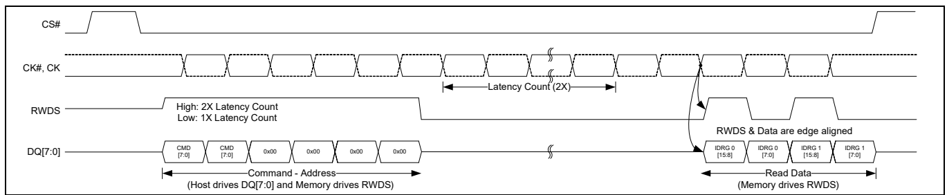
Figure 8 READ ID with 2X latency transaction (DDR) [14]
