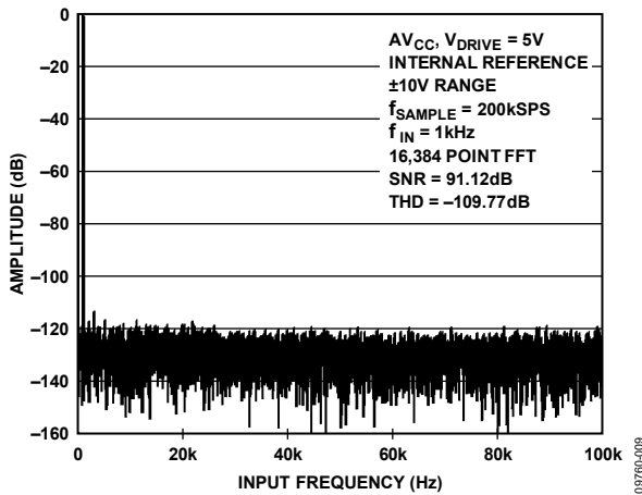
Figure 9. FFT Plot, ±10 V Range
