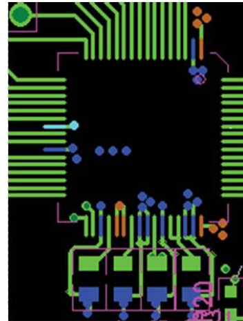
Figure 60. Top Layer Decoupling REFIN/REFOUT, REFCAPA, REFCAPB, and REGCAP Pins
