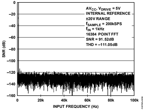
Figure 8. FFT Plot, ±20 V Range
