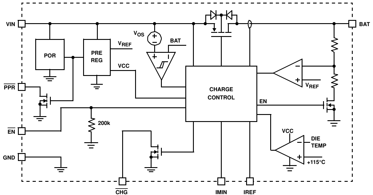
FIGURE 3. BLOCK DIAGRAM
