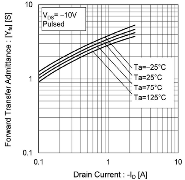
Fig.6 Forward Transfer Admittance vs. Drain Current
