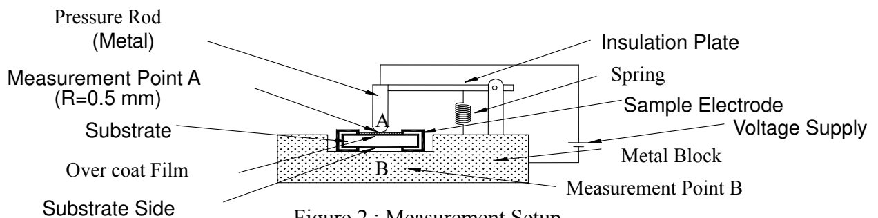
Figure 2 : Measurement Setup
