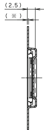
SECT. E-E (22~30P)
