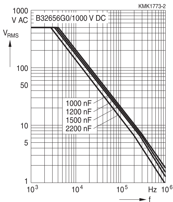
1000 V DC/500 V AC, B32656G0
