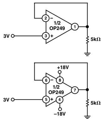
Figure 5. Burn-In Circuit
