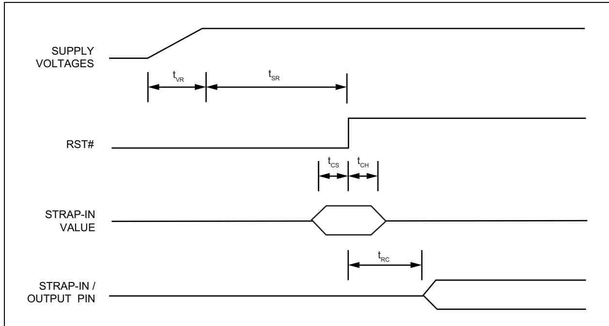
FIGURE 7-15: RESET TIMING
