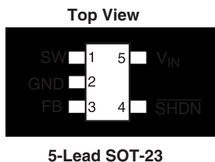
Figure 2. Pin Assignment
