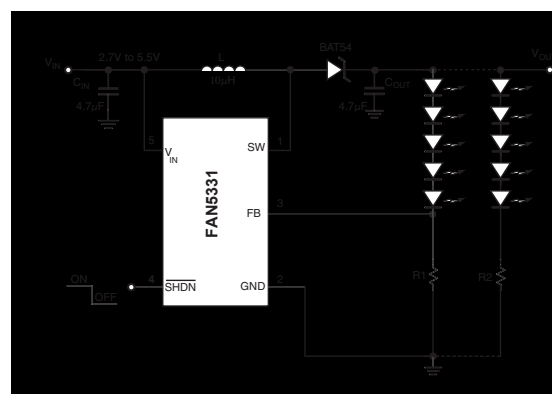
Figure 6. Low Noise Boost LED Driver
