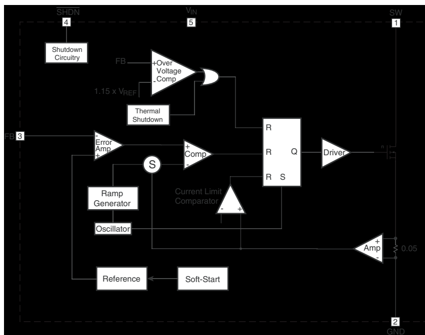
Figure 4. Block Diagram
