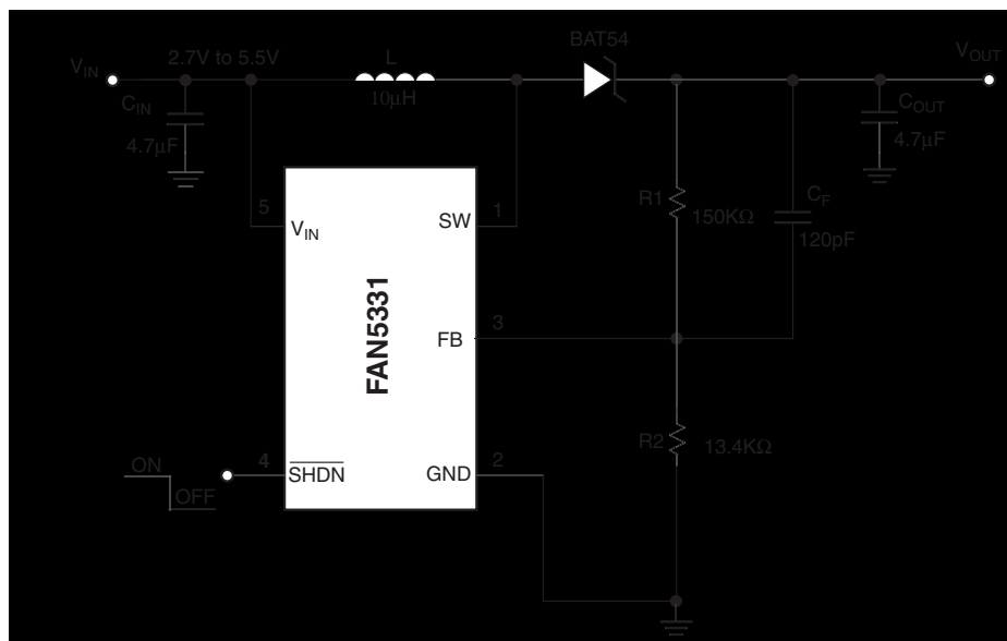
Figure 3. Test Circuit
