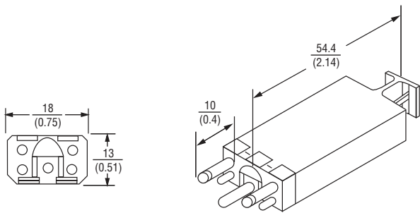
Figure 3 12A-Type Protector
