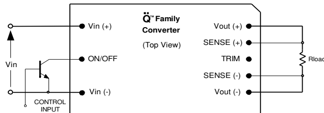
Figure 1. Circuit configuration for ON/OFF function.
