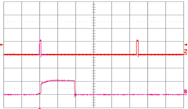
Figure 25. Load current (top trace, 20 A/div, 20 ms/div) into a 10 mΩ short circuit during restart, at Vin = 24 V. Bottom trace (20 A/div, 1 ms/div) is an expansion of the on-time portion of the top trace.
