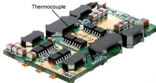
Figure 26. Location of the thermocouple for thermal testing.
