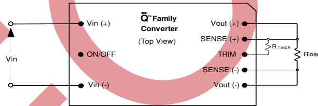
Figure 3. Configuration for increasing output voltage.
