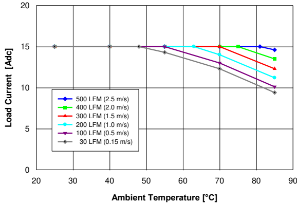
Figure 8. Available load current vs. ambient air temperature and airflow rates for converter mounted vertically with V_{in} = 27\text{ V} , air flowing from pin 3 to pin 1 and maximum FET temperature \leq 120\text{ }^{\circ}\text{C} .
