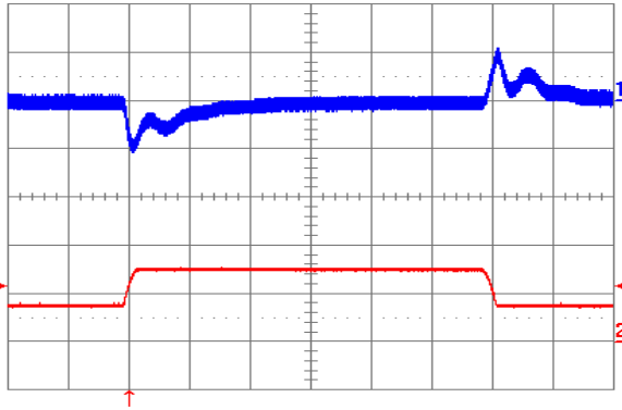
Figure 18. Output voltage response to load current step-change (3.75 A – 7.5 A – 3.75 A) at V_{in} = 24 V. Top trace: output voltage (100 mV/div). Bottom trace: load current (5 A/div.). Current slew rate: 0.1 A/ \mu s. C_o = 1 \mu F ceramic. Time scale: 0.2 ms/div.
