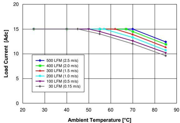
Figure 10. Available load current vs. ambient temperature and airflow rates for converter mounted horizontally with V_{in} = 27\text{ V} , air flowing from pin 3 to pin 4 and maximum FET temperature \leq 120\text{ }^{\circ}\text{C} .
