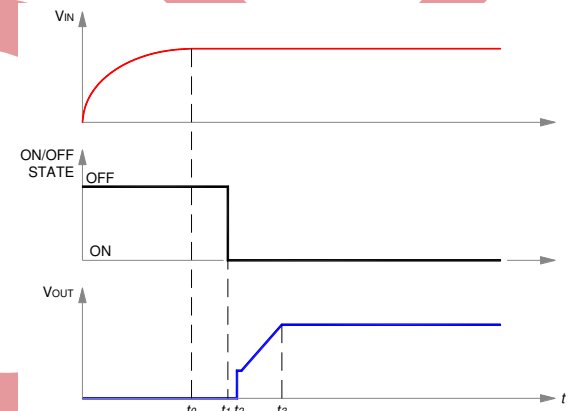
Figure 6. Startup scenario #2.
