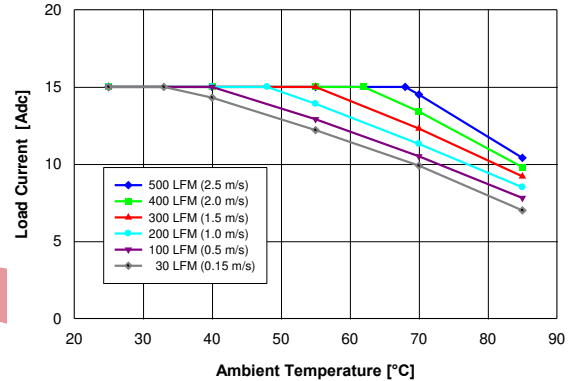
Figure 9. Available load current vs. ambient air temperature and airflow rates for converter mounted vertically with V_{in} = 27\text{ V} , air flowing from pin 3 to pin 1 and maximum FET temperature \leq 105\text{ }^{\circ}\text{C} .
