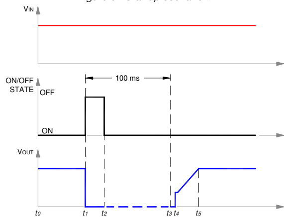
Figure 7. Startup scenario #3.
