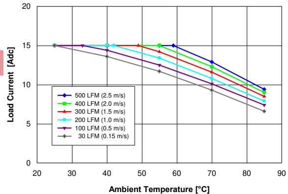
Figure 11. Available load current vs. ambient temperature and airflow rates for converter mounted horizontally with V_{in} = 27\text{ V} , air flowing from pin 3 to pin 4 and maximum FET temperature \leq 105\text{ }^{\circ}\text{C} .
