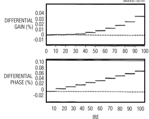
DIFFERENTIAL GAIN AND PHASE ( R_L = 1k\Omega )
