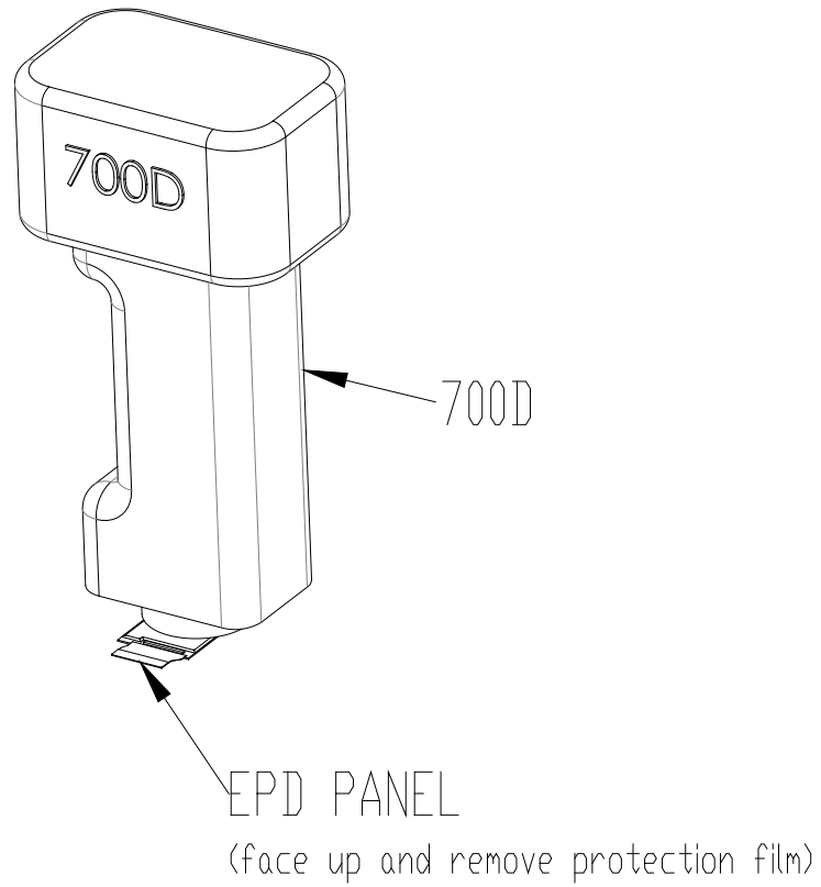
Figure 6-1 Optical measurement
