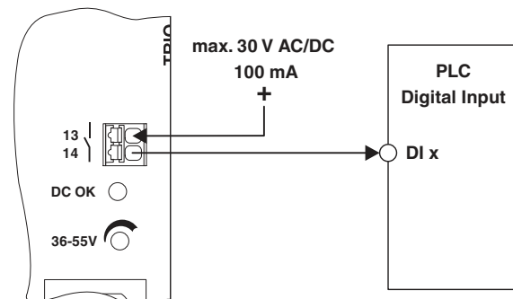
Figure 19 Wiring principle
