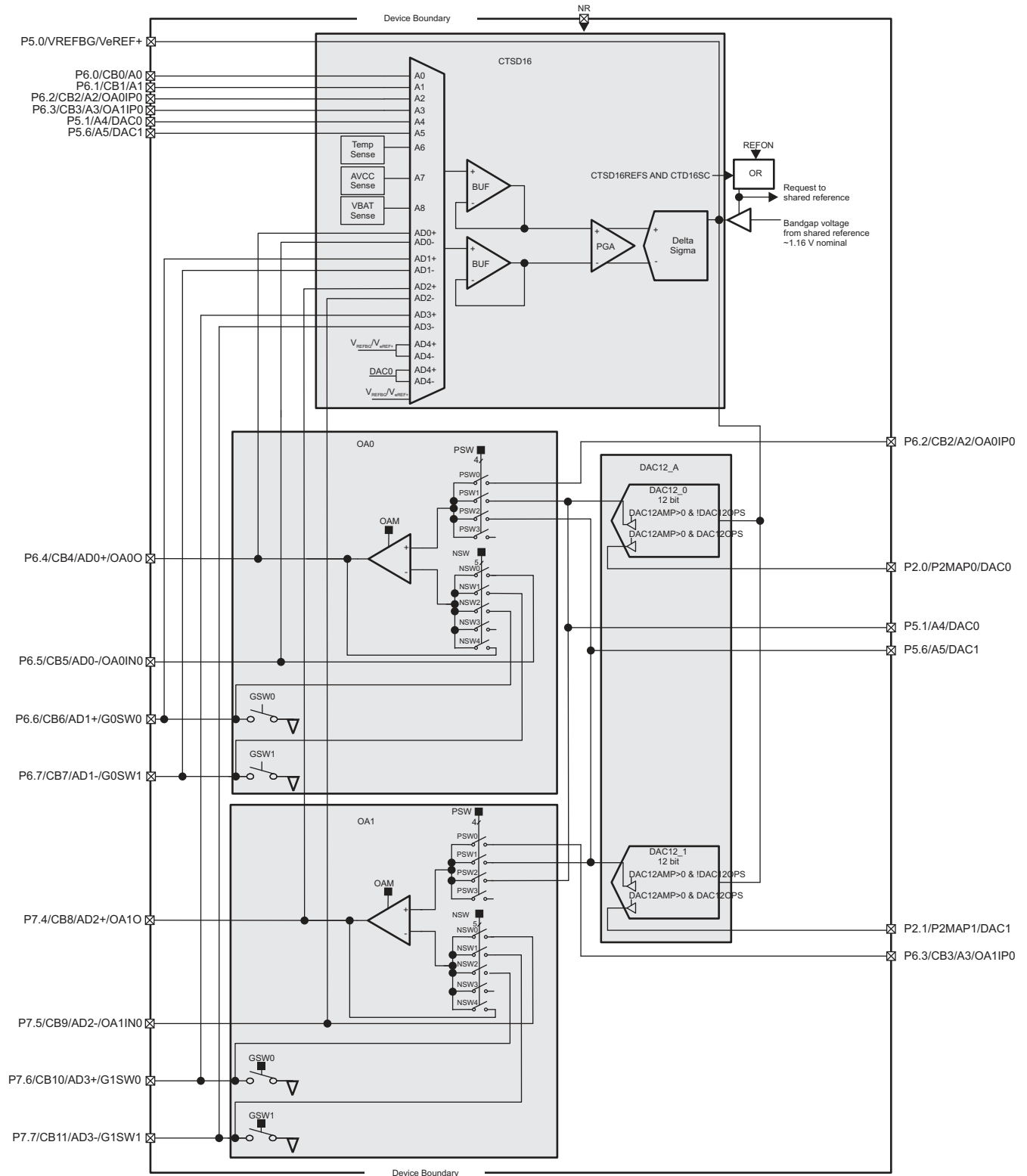
Figure 9-2. Signal Chain
