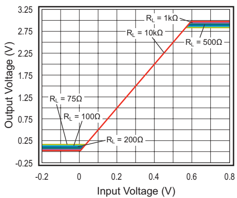
Figure 20. Output Voltage Swing vs. Load (3V)
