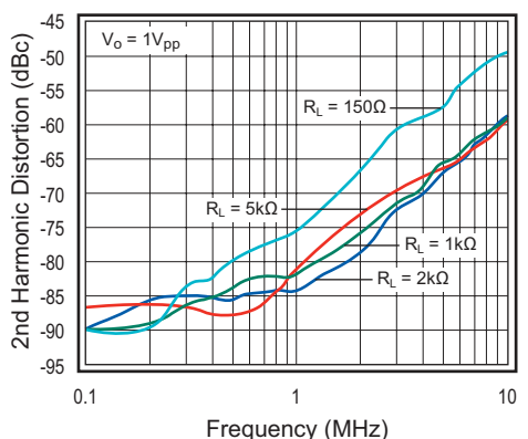
Figure 14. HD2 vs. R_L (3V)
