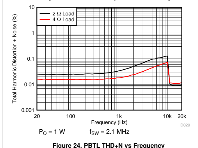
Figure 24. PBTLD THD+N vs Frequency
