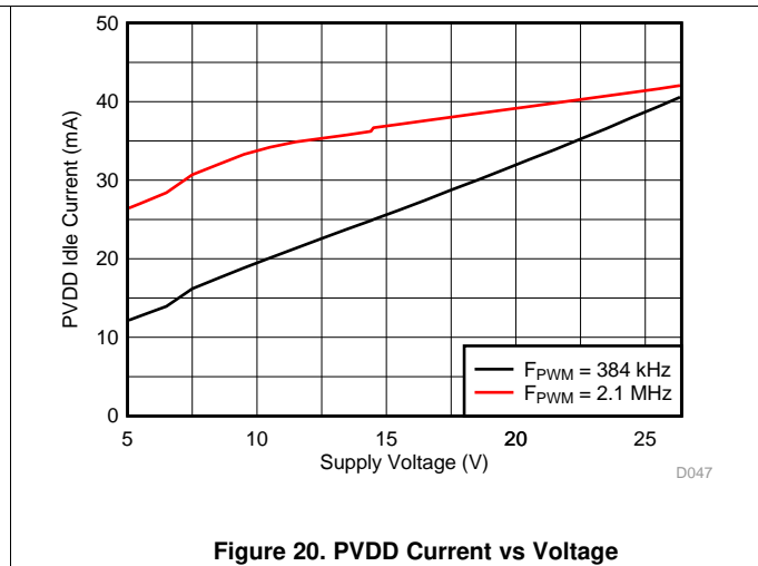
Figure 20. PVDD Current vs Voltage
