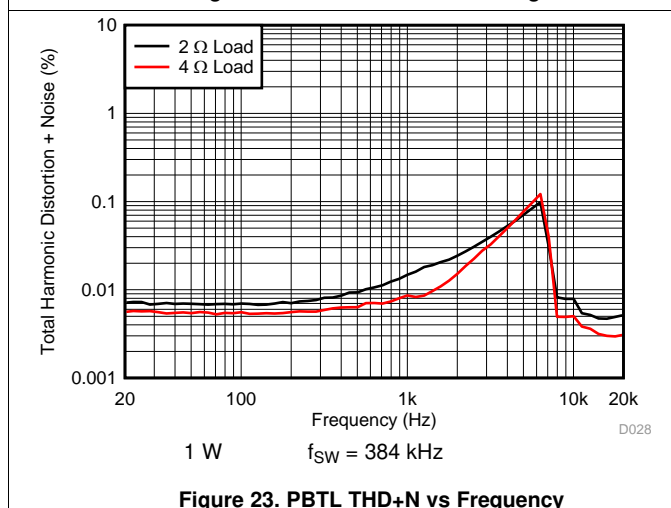
Figure 23. PBTLD THD+N vs Frequency
