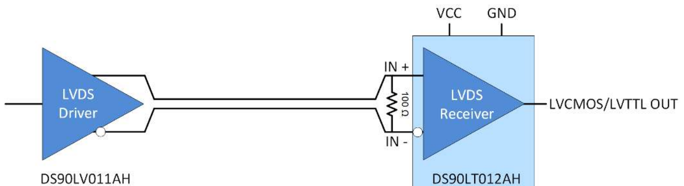
Figure 12. Typical Application
