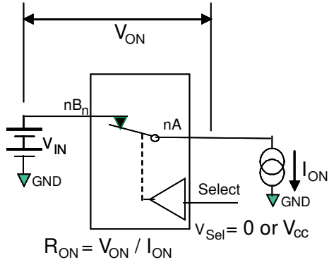
Figure 5. On Resistance
