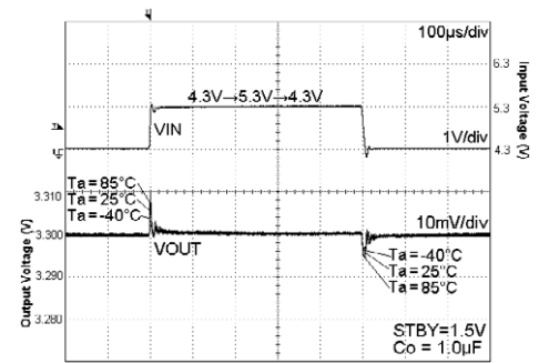
Fig. 39 VIN Response Iout = 10mA
