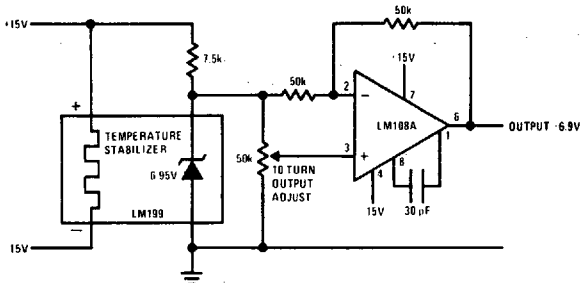
Voltage Reference
